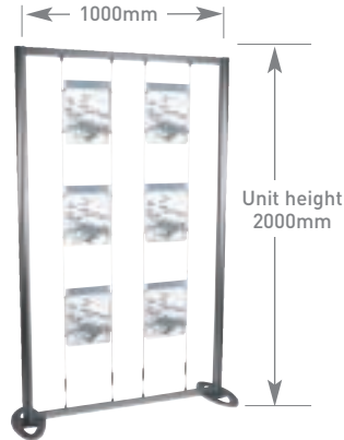
Kit 3 (6 x A4 holders) Additional wire kit accessories available.
